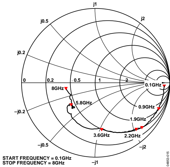
Figure 15. Input Impedance vs. Frequency; No Termination Resistor on INHI
